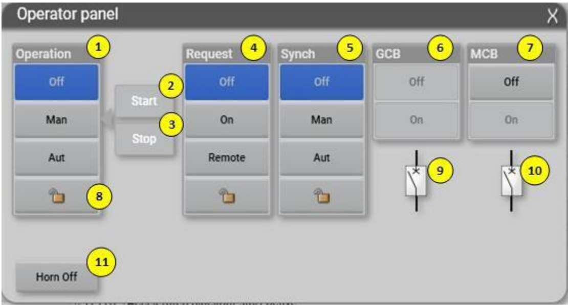
Figure 4: INNIO J620/J624 Operator Panel
